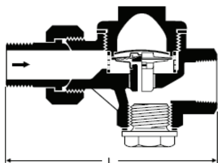
МК 20, DN 15, 20 mm
