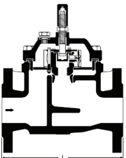
TK, DN 50, 65, 80, 100 mm
