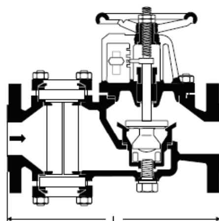
GK 11, DN 65, 80, 100, 150 mm GK 21, DN 50 mm
